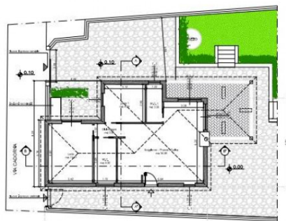
PLANIMETRIA PIANO TERRA RAPP. 1 : 100
