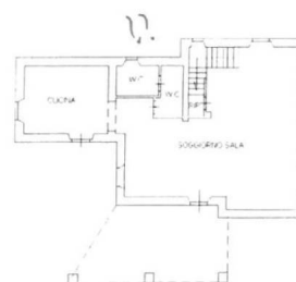
PIANO TERRA-H=2.70
